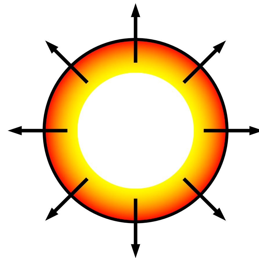
detonation
