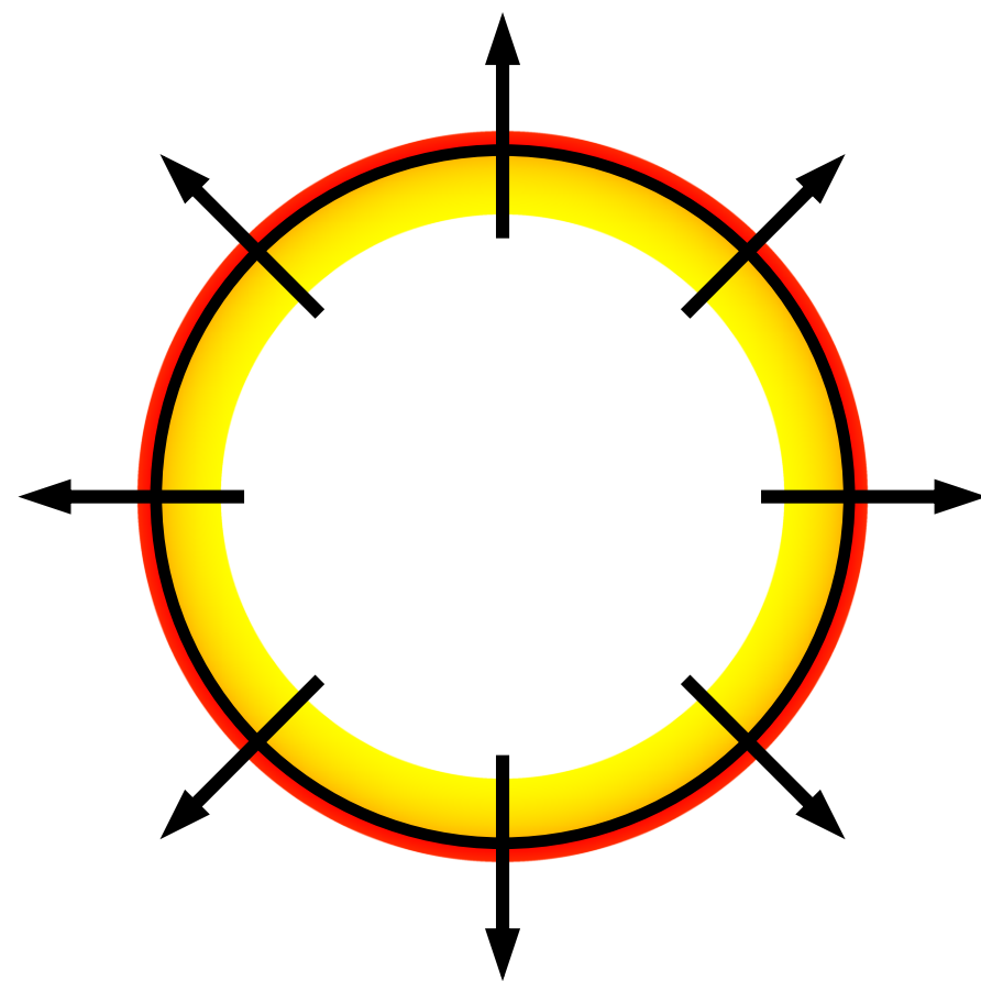
supersonic deflagration
