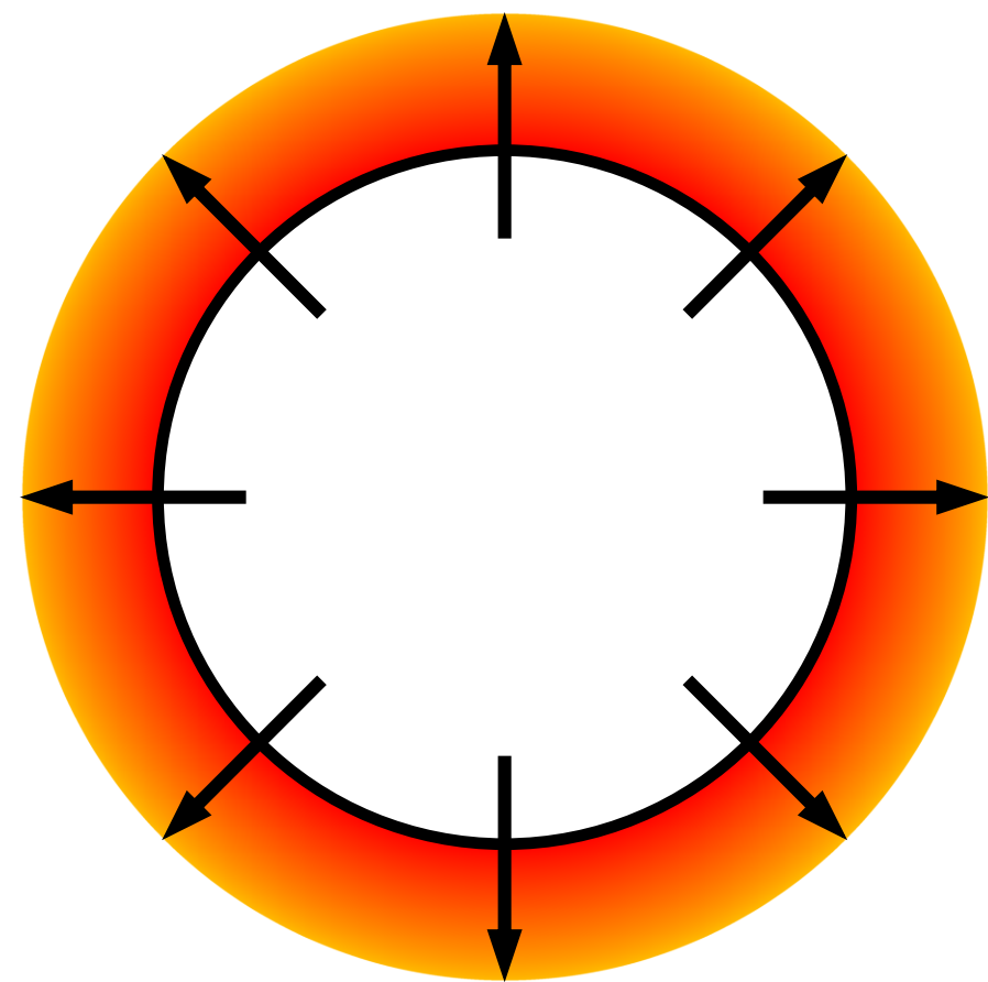
subsonic deflagration
